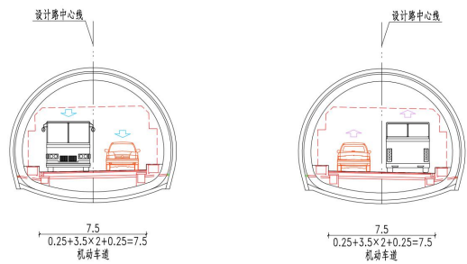
隧道段横断面图
